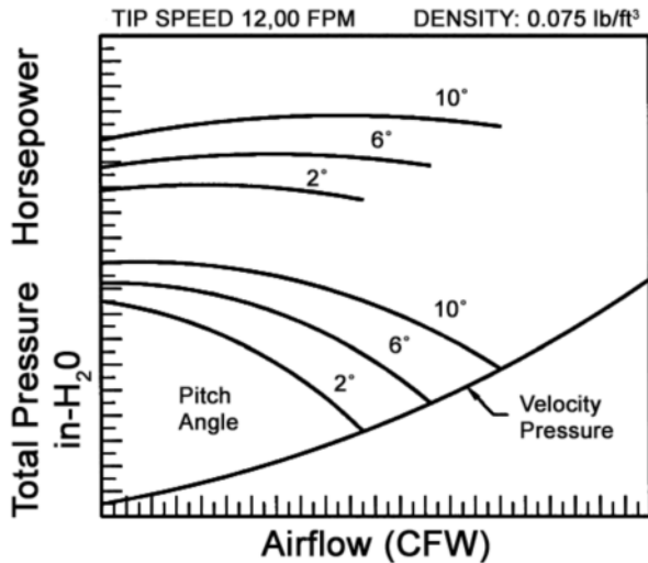
Typical Fan Curve Fig. 2
