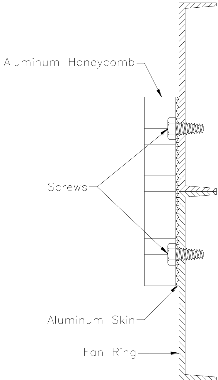
Figure 1 - Tip Seal
